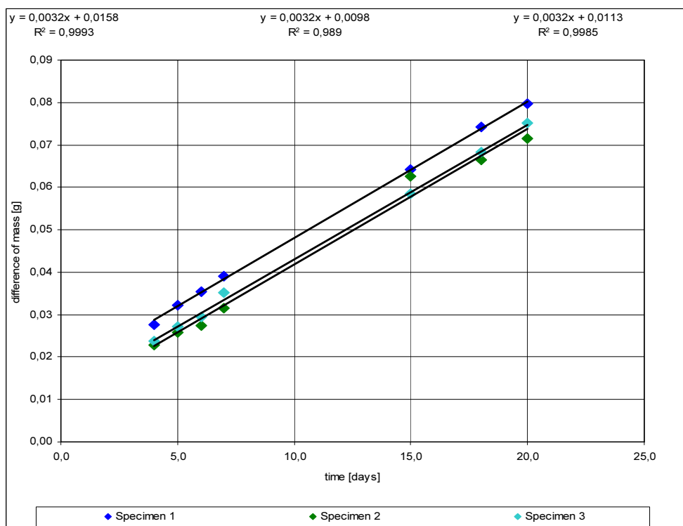
Fig. 6 Graph of the moisture vapour transmission rate of 3 test specimen
