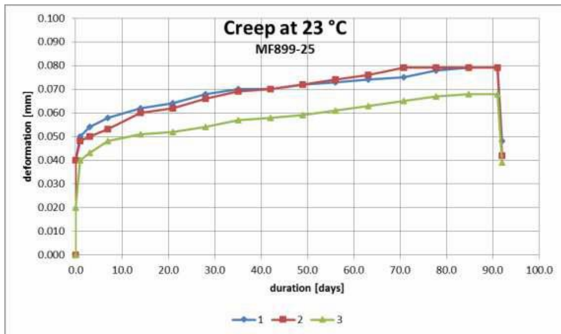
Figure 3: Creep sealant MF899-25 at 23°C
