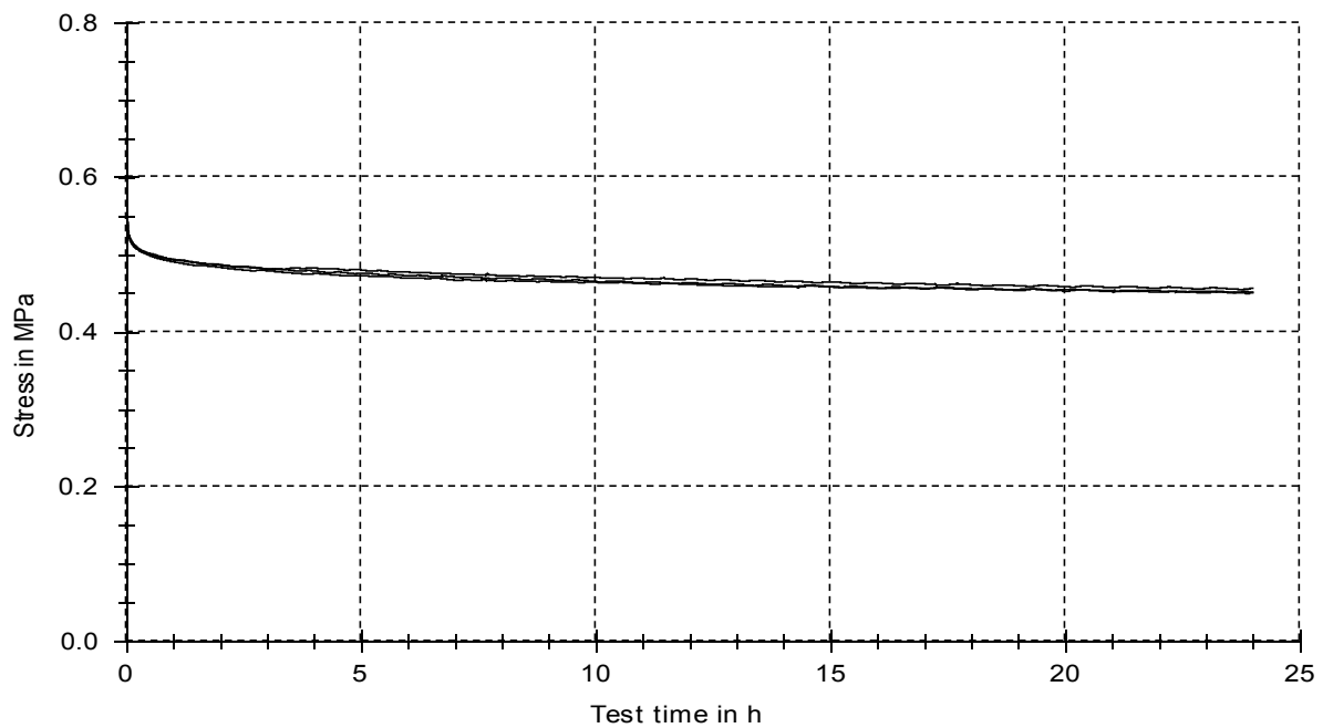
Figure 2: Elastic relaxation curve MF899-25 at 25 % extension.
