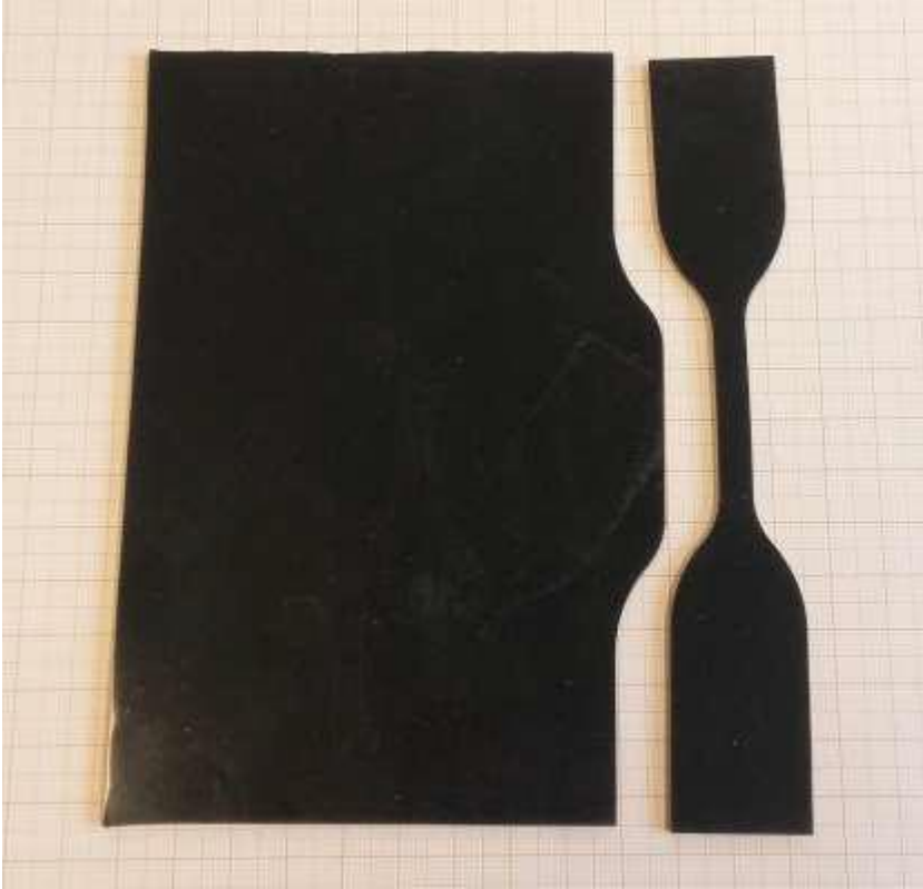
Sample type 2 and ISO 527 type 5 specimens punched from 2 mm sealant film
