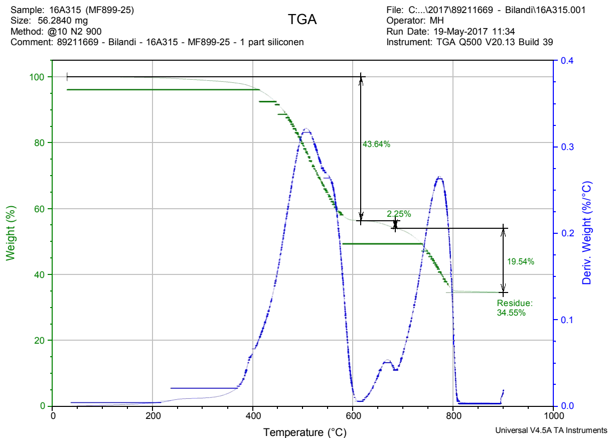
Figure 2: TGA curve, weight loss of MF889-25 Silicone structural sealant up to 900 °C.
