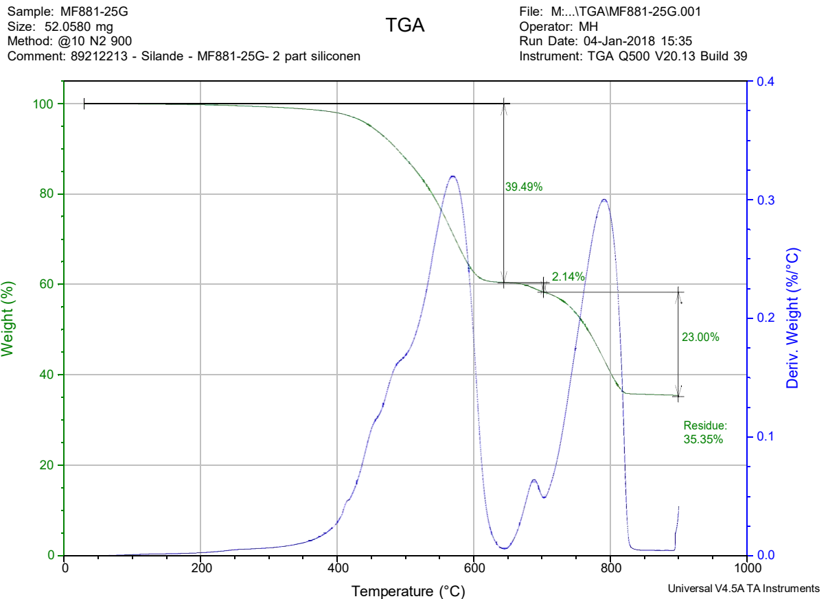
Figure 2: TGA curve. weight loss of MF881-25G Silicone Structural Sealant up to 900 °C.
