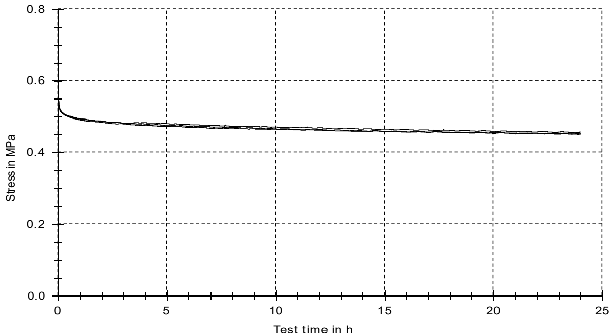
Figure 2: Elastic relaxation curve MF881-25G at 25 % extension.
