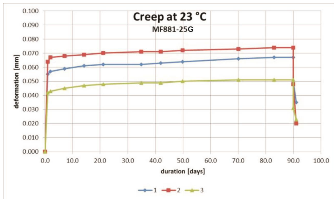
Figure 3: Creep sealant MF881-25G at 23°C
